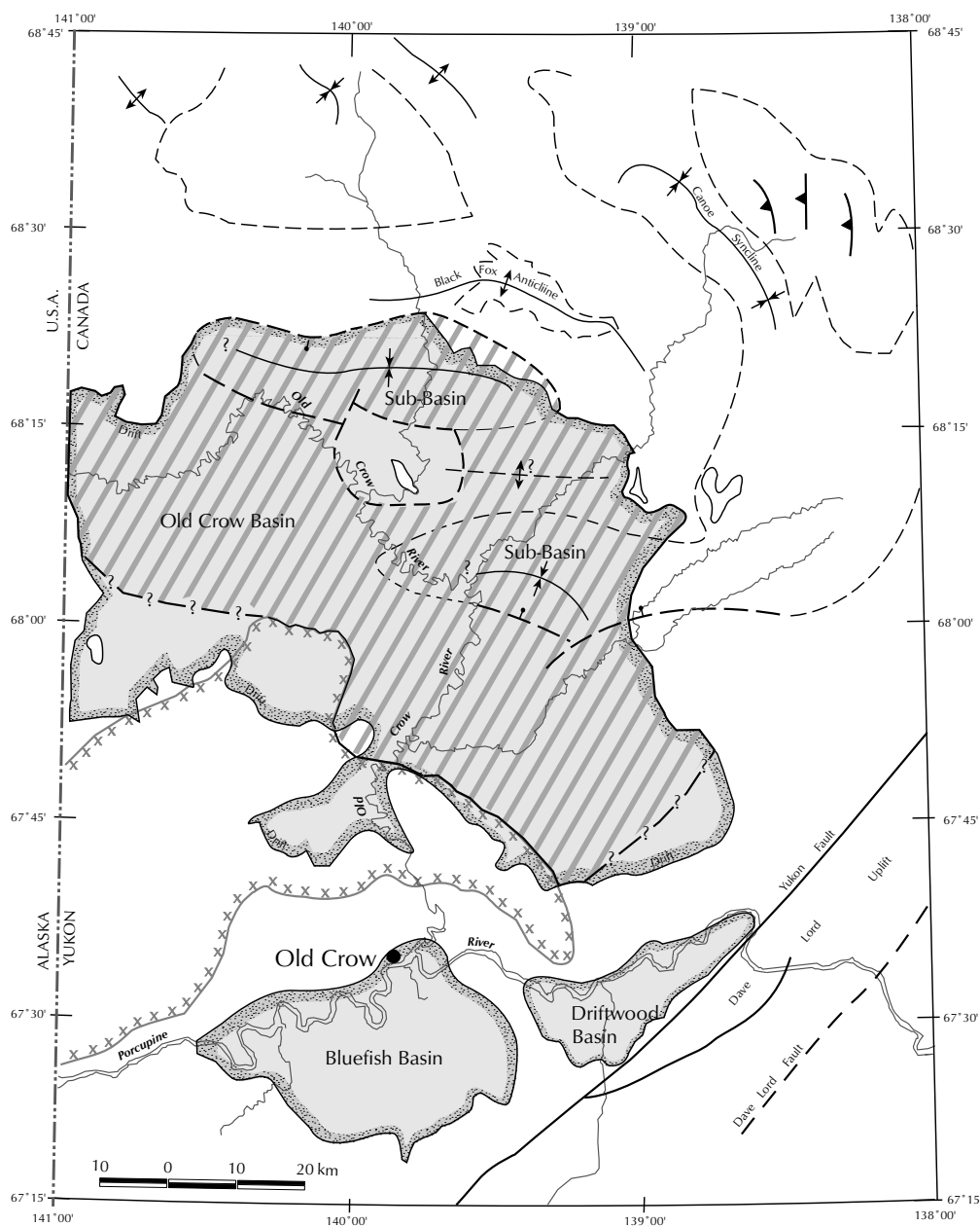
Figure 15. Upper Paleozoic carbonate gas play.
